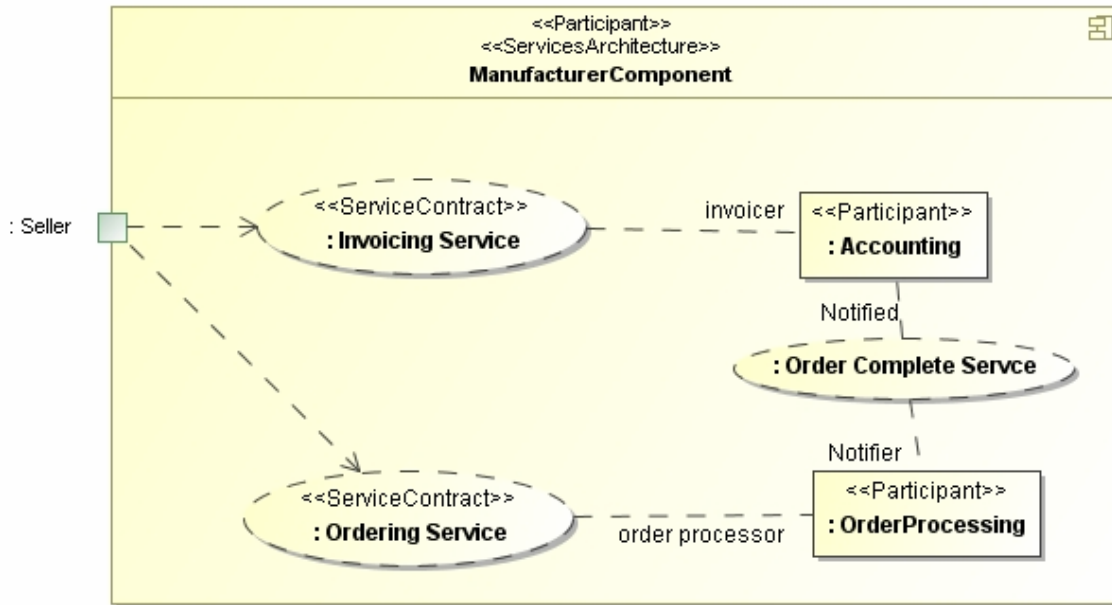
Figure 45: Participant’s services architecture
