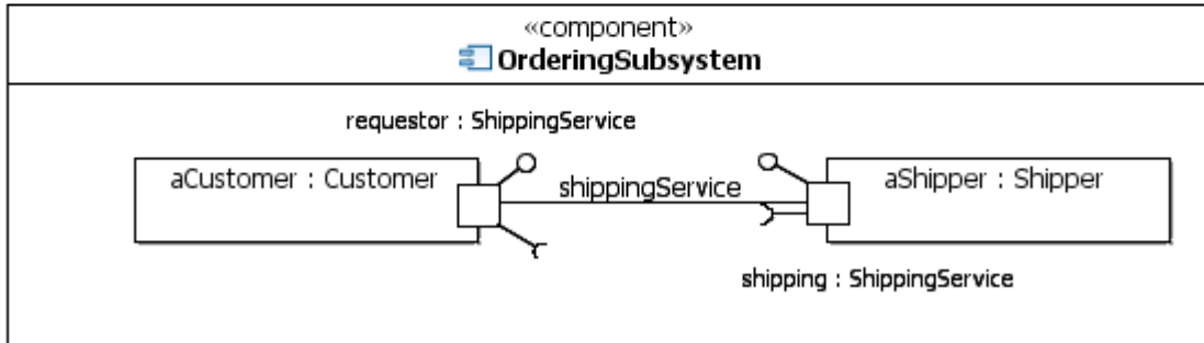
Figure 42: Using the shipping Service with one Consumer
