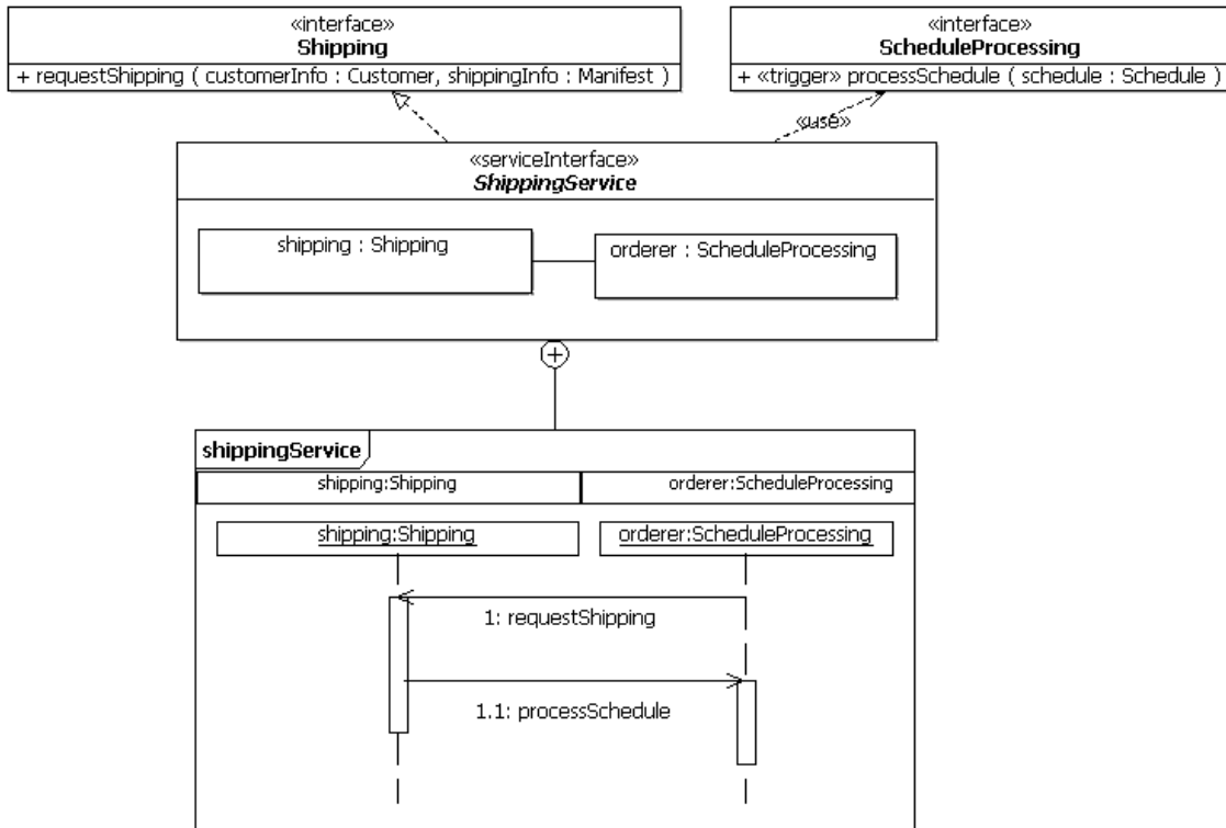
Figure 111: ShippingService Service Interface
