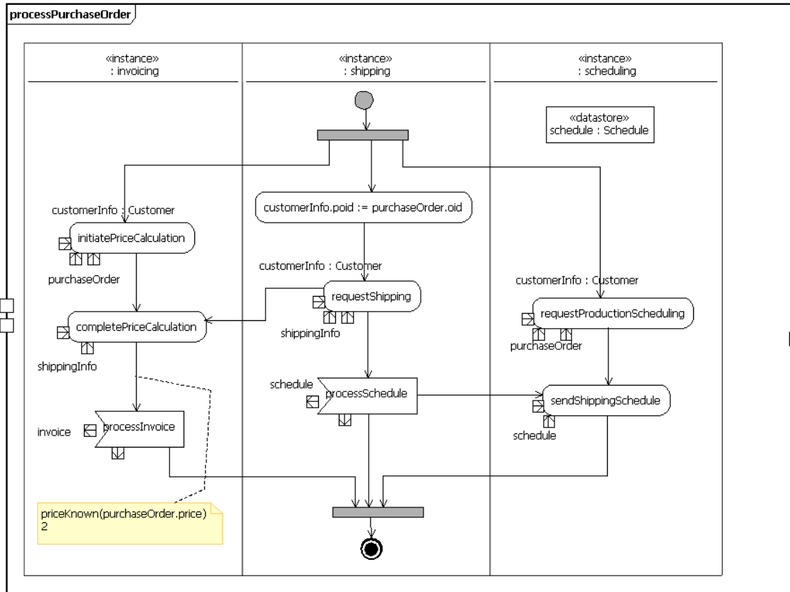
Figure 119: The processPurchaseOrder Service Operation Design
