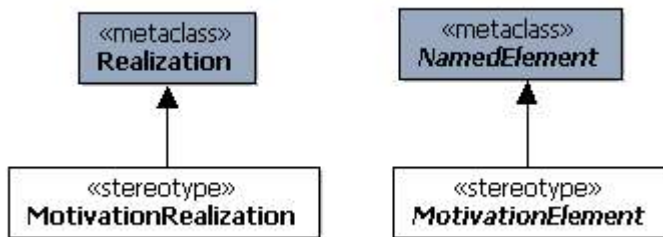
Figure 52: The BMM Integration Profile Elements
