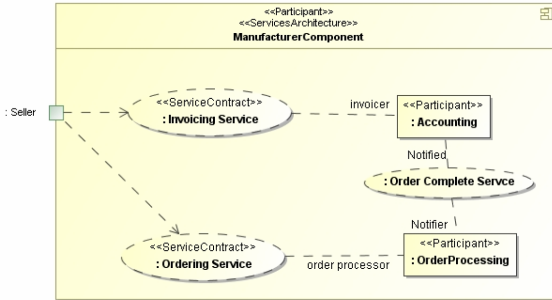
Figure 8: Example Services architecture for a participant
