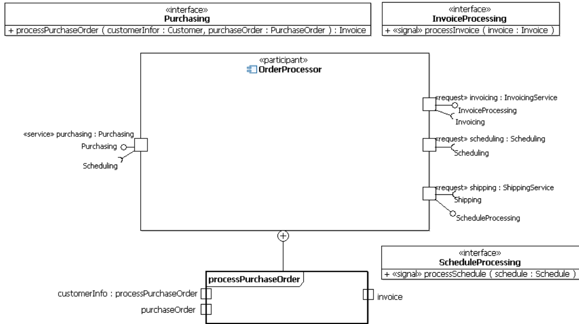
Figure 25: The OrderProcessor Participant
