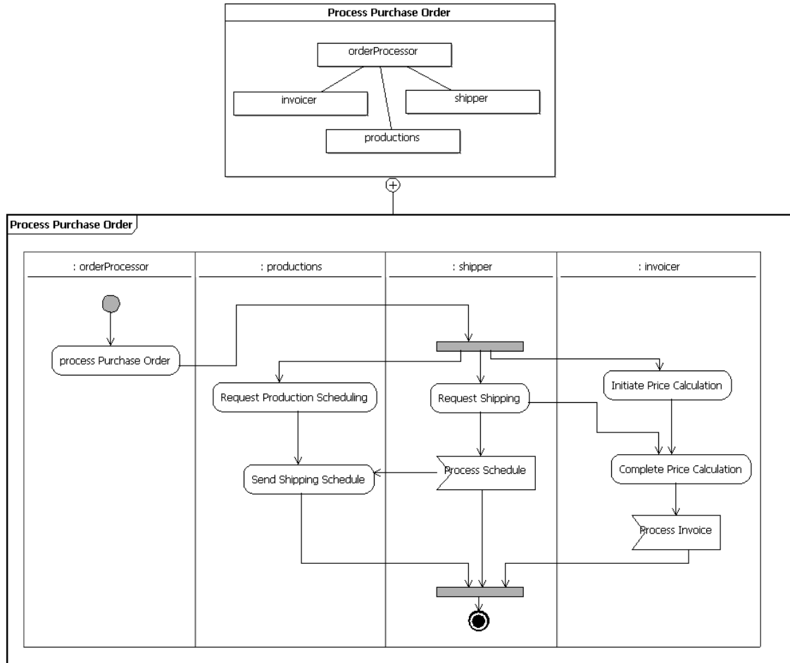
Figure 106: Process Purchase Order Contract
