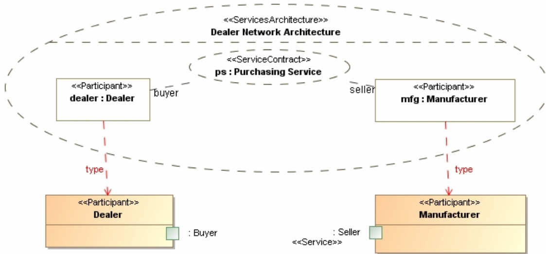
Figure 44: Abbreviated service contract
