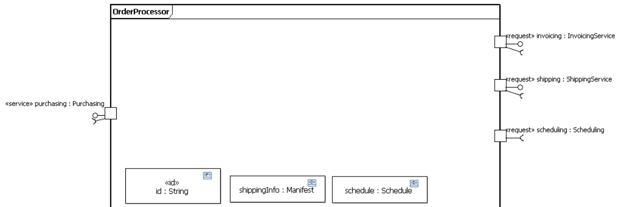
Figure 29: Requests of the OrderProcessor Participant
