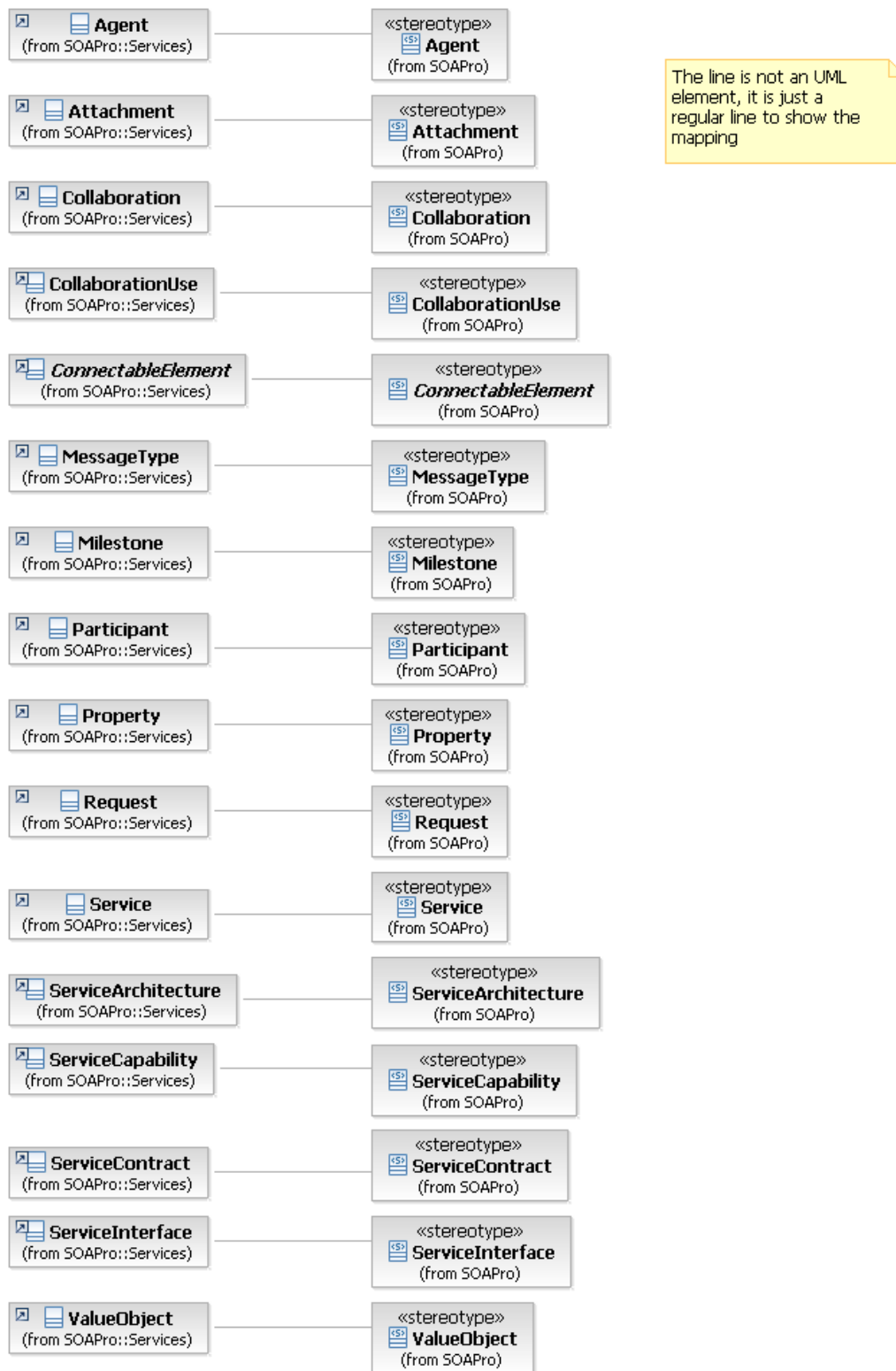
Figure 96: Profile metamodel mapping
