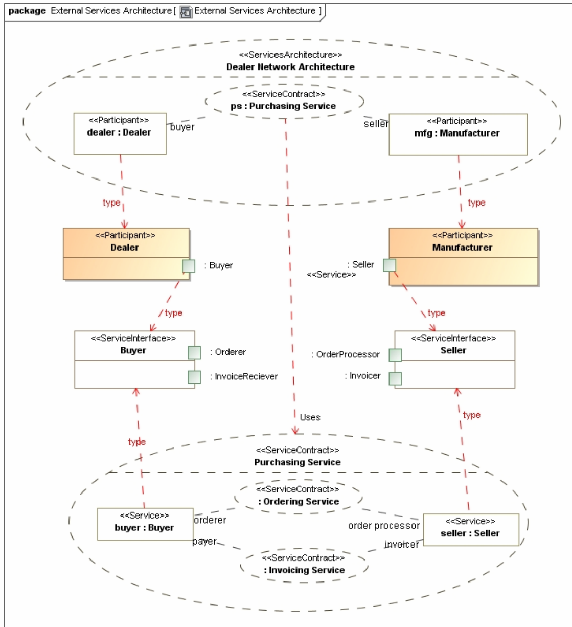
Figure 105: Relating services architecture as service contracts
