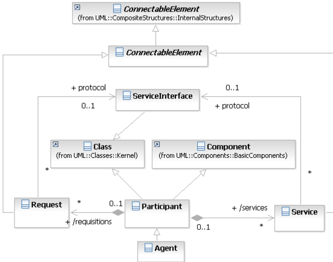
Figure 55: ServiceInterfaces and Participants
