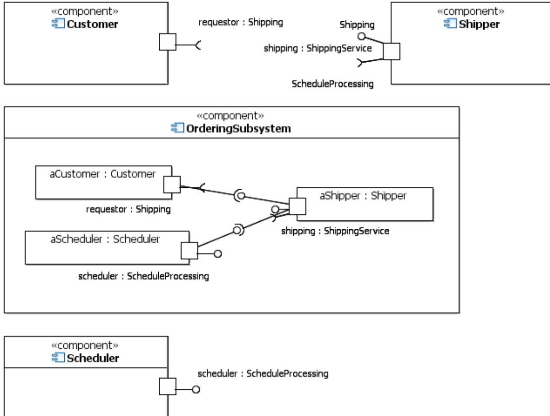
Figure 41: Using the shipping Service with two Consumers
