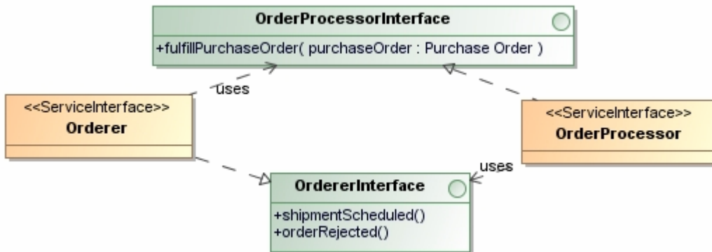
Figure 35: Service interfaces that correspond to the above
