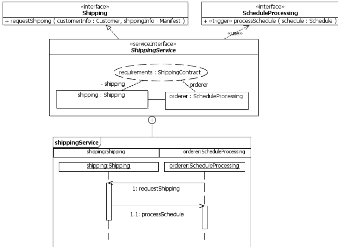
Figure 20: Fulfilling the ShippingContract ServiceContract
