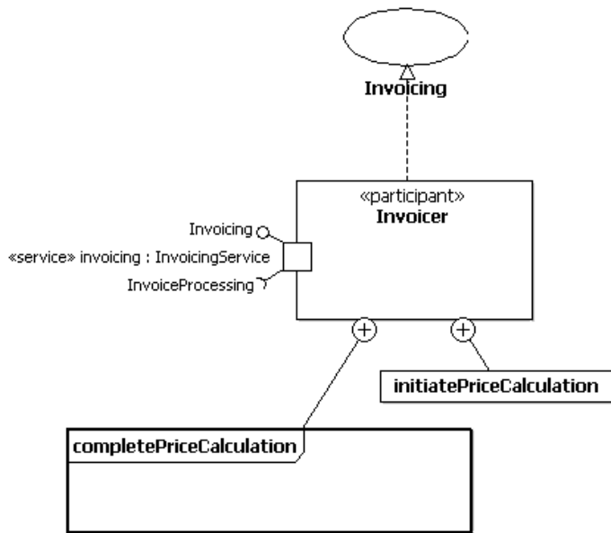
Figure 30: The invoicing Service of the Invoicer Participant
