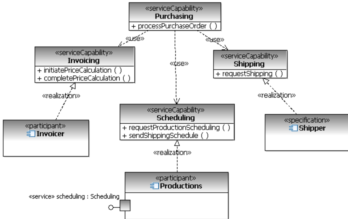
Figure 12: Realizing the order processing service capabilities
