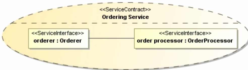
Figure 99: Ordering service
