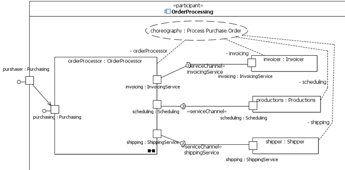
Figure 32: The OrderProcessing Participant
