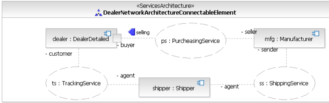
Figure 92: Diagram 04. ContractsConnectableElement
