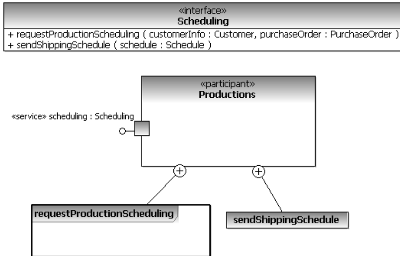
Figure 3: Services and Service Participants
