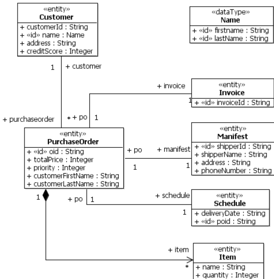
Figure 28: Example entities from the CRM domain model
