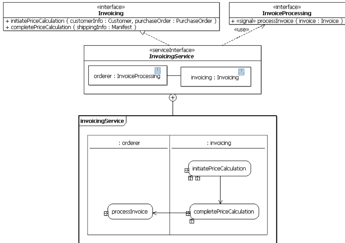
Figure 109: InvoicingService Service Interface
