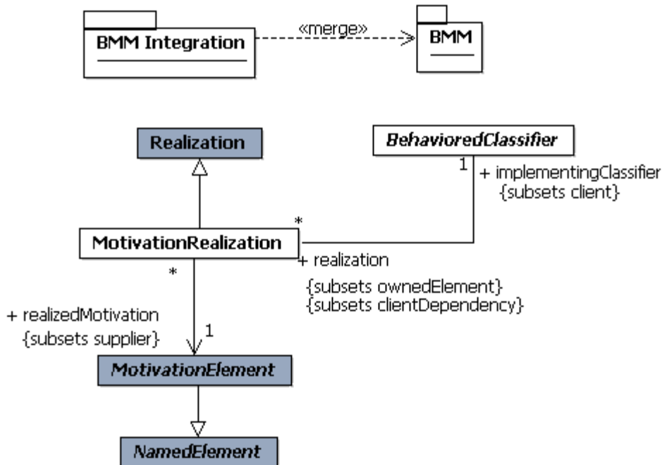
Figure 53: BMM Integration Package
