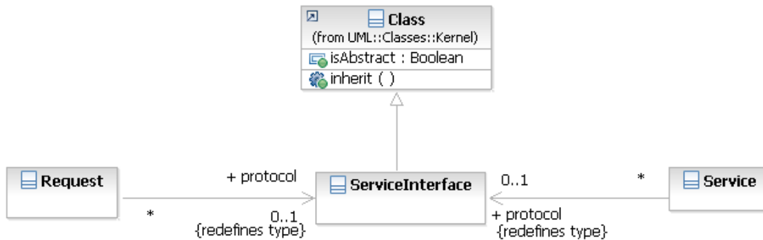
Figure 87: ServiceInterface
