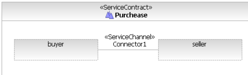
Figure 86: Diagram 05. ConstraintsAndObjectives
