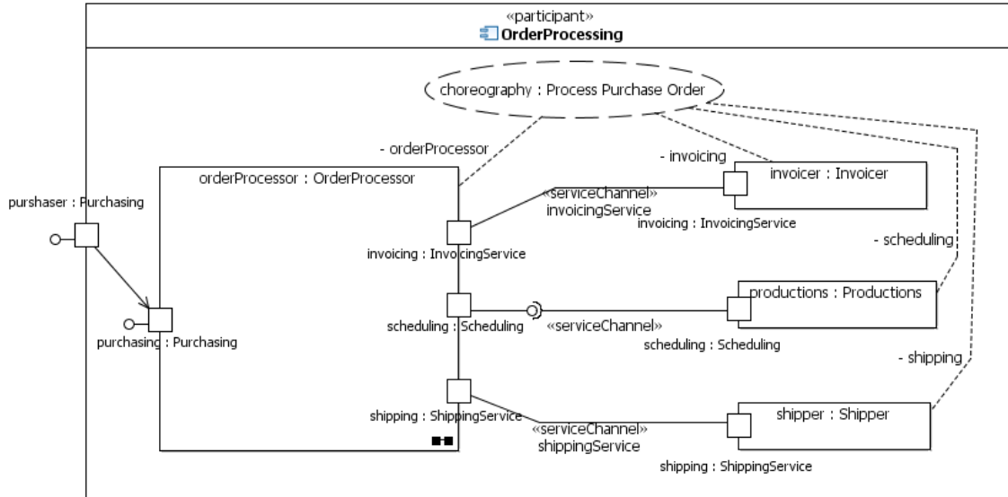
Figure 21: Fulfilling the Process Purchase Order Contract
